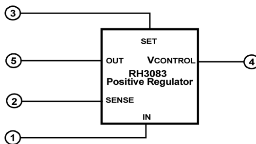
Figure 1 - Block Diagram / Schematic
